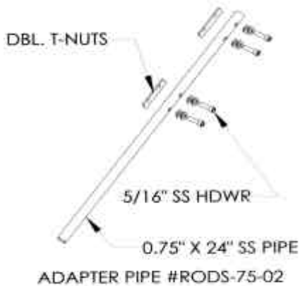
ADAPTER PIPE #RODS-75-02
