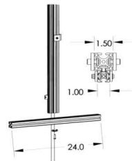
1.5" DUAL BASE RAIL #LNCH-15-05
